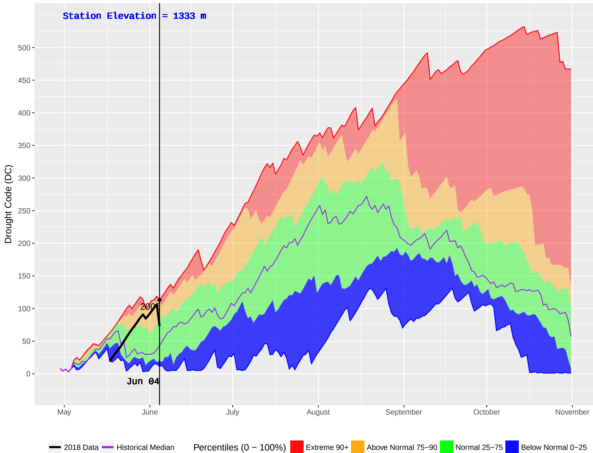
GOLDSTREAM 2 (919) : Historical (2005–2016) and Current (2018) Noon Drought Code (DC)
