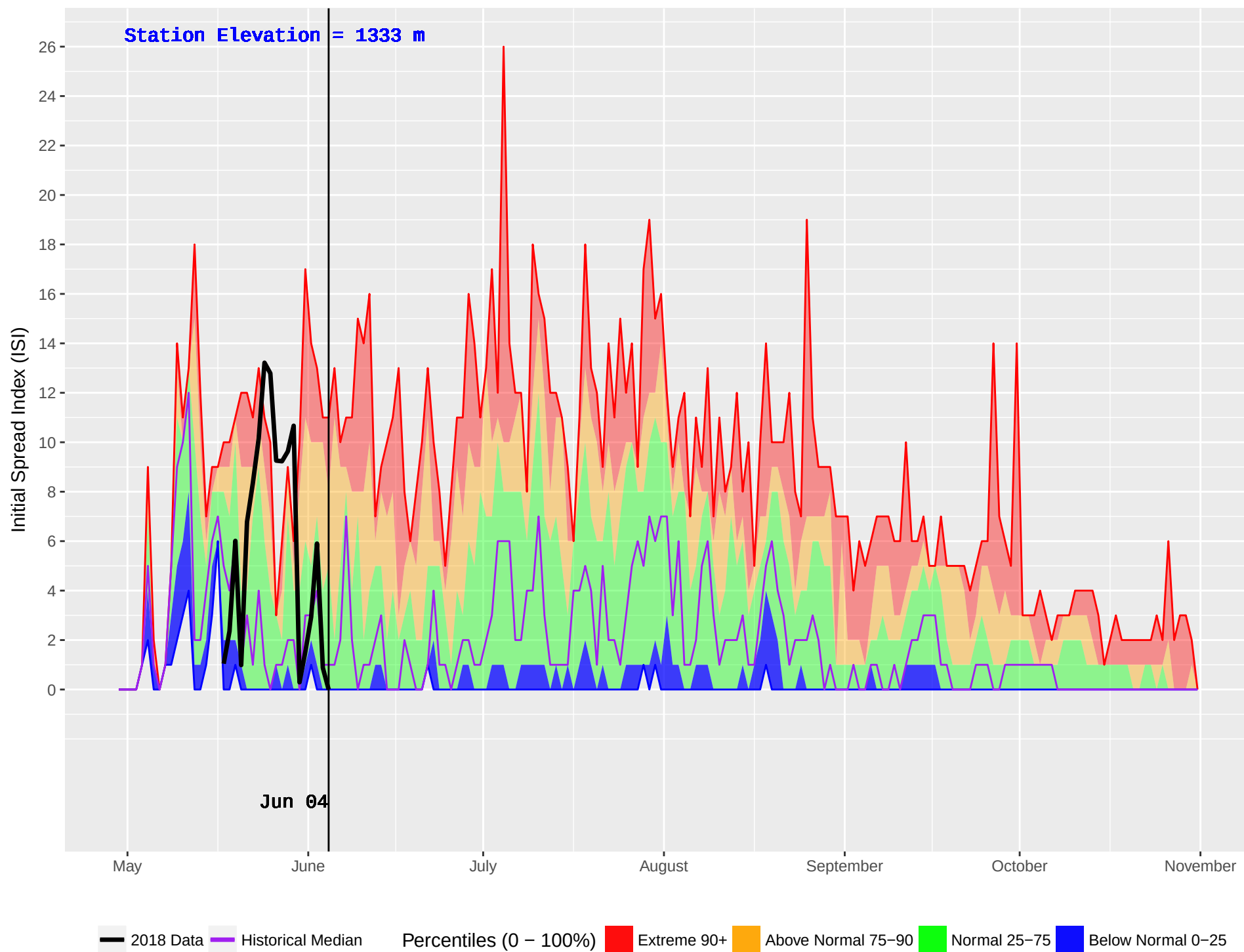
GOLDSTREAM 2 (919) : Historical (2005–2016) and Current (2018) Noon Initial Spread Index (ISI)
