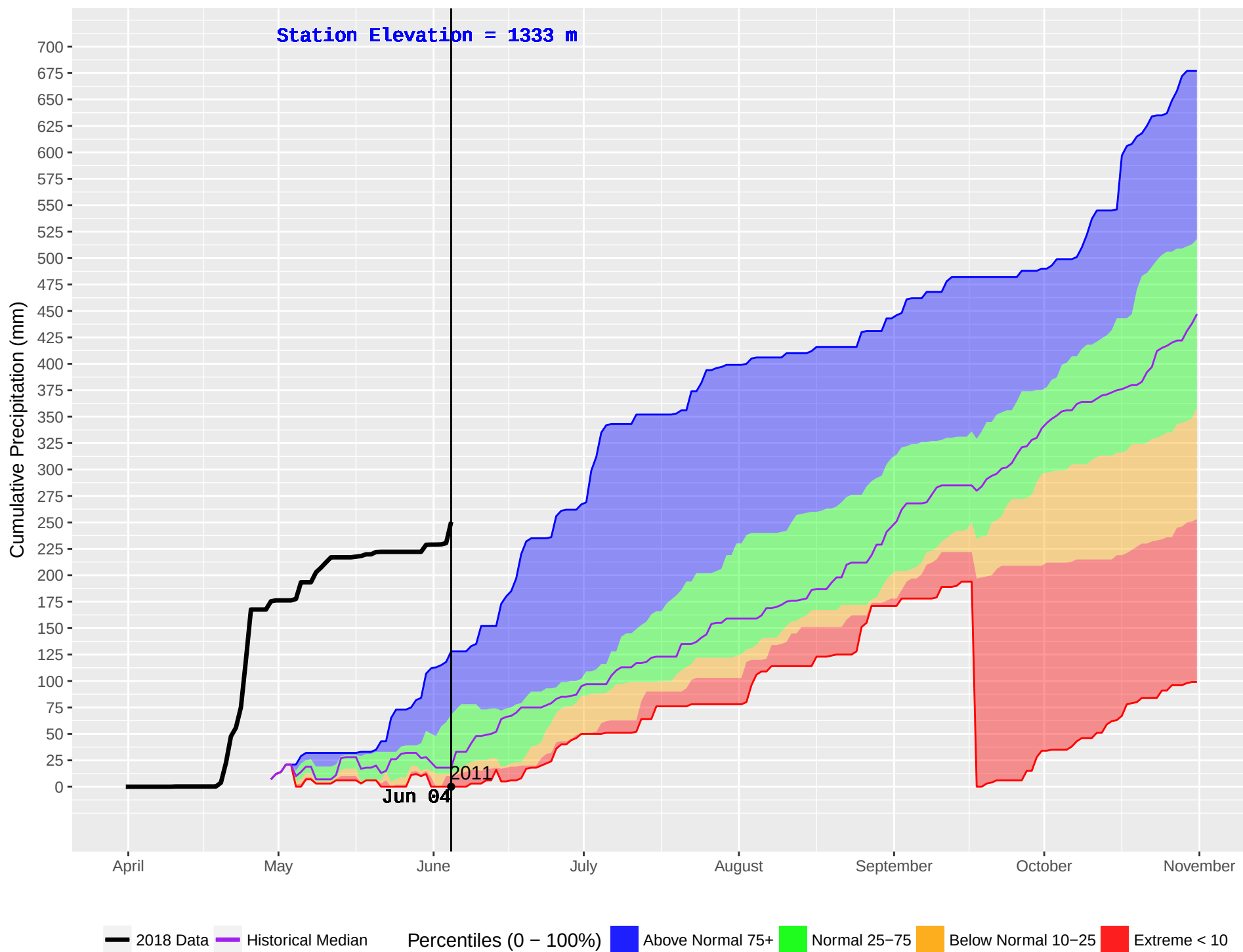
GOLDSTREAM 2 (919) : Historical (2005–2016) and Current (2018) Noon Cumulative Precipitation
