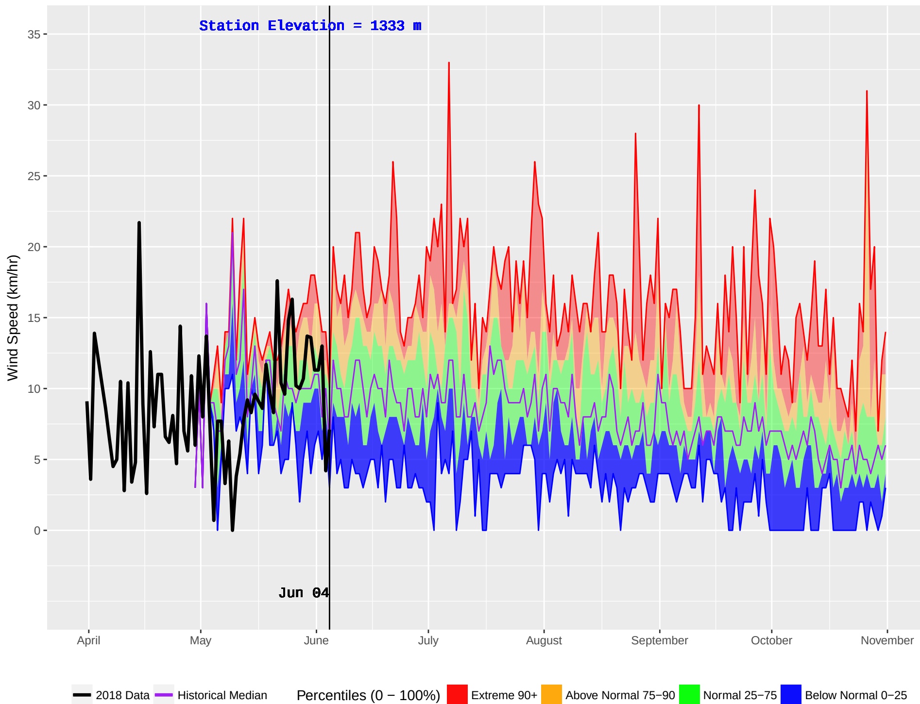
GOLDSTREAM 2 (919) : Historical (2005–2016) and Current (2018) Noon Wind Speed
