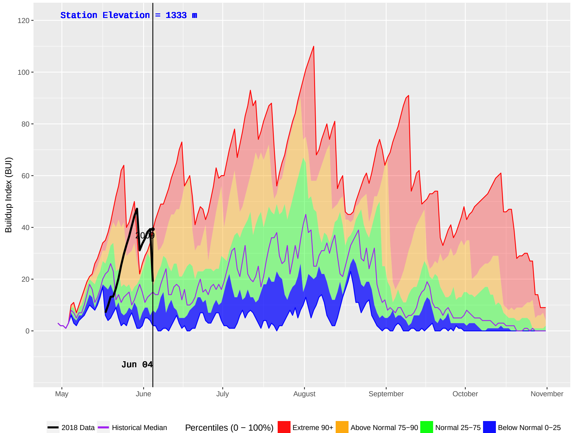
GOLDSTREAM 2 (919) : Historical (2005–2016) and Current (2018) Noon Buildup Index (BUI)
