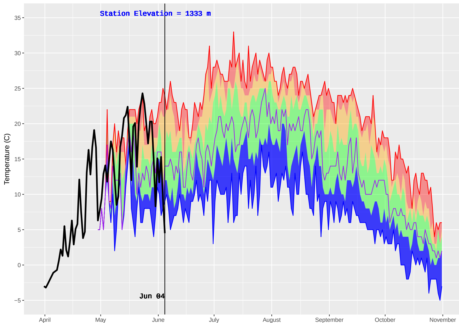
GOLDSTREAM 2 (919) : Historical (2005–2016) and Current (2018) Noon Temperature
